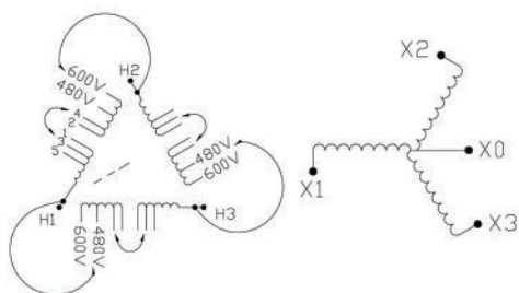
Schematic
