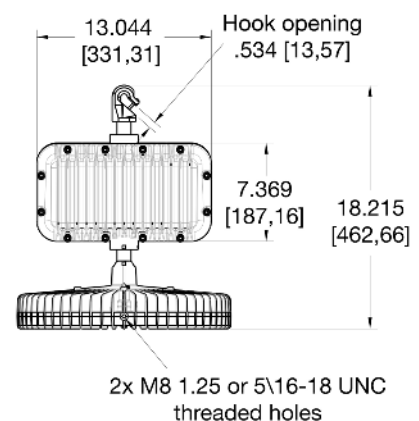
HBXH - Hook
