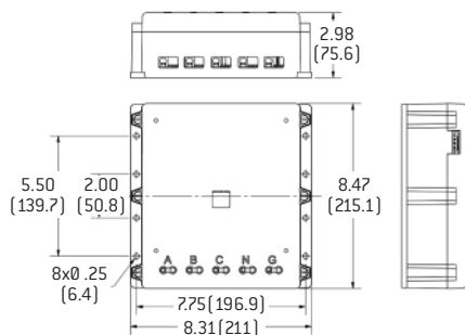
Option Q (Does not include HMI)
