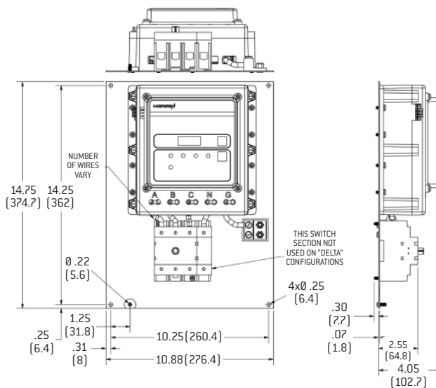
Option Q - With Disconnect Switch
