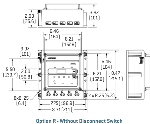
Option R - Without Disconnect Switch
